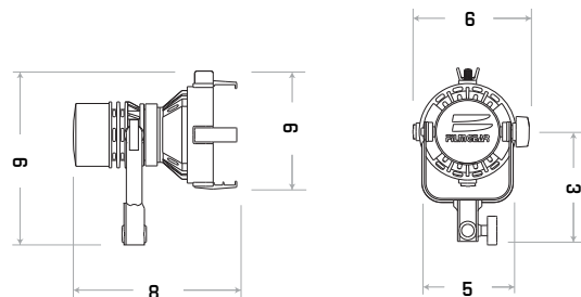
Daylight Boxer with Reflector
